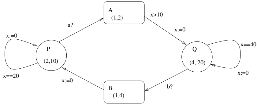
Fig. 5. Timed Automaton with Periodic and Sporadic Tasks.
