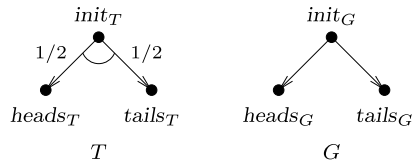
Fig. 1. T tosses a coin and G has to guess.
