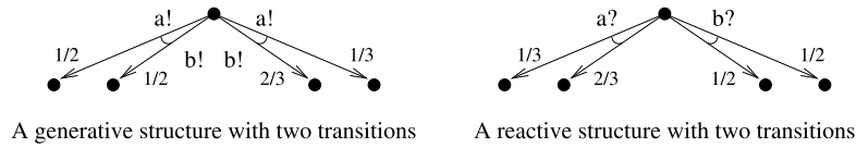
Fig. 2. Reactive and generative structures.
