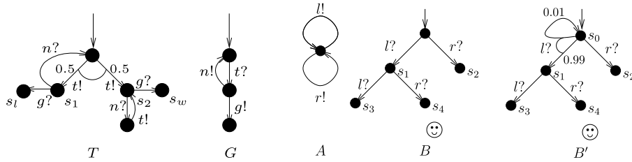
Fig. 5. Atoms used in our examples.
