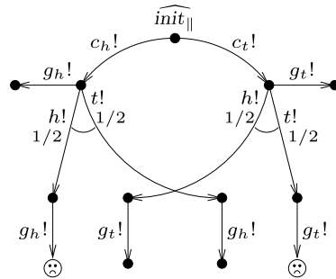
Fig. 14. A POR based reduction.
