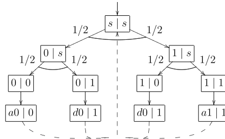
Fig. 9. Unrealistic counterexample in the parallel composition.
