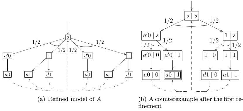
Fig. 10. Refined system and counterexample.
