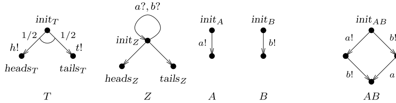
Fig. 3. Motivating strongly distributed schedulers.
