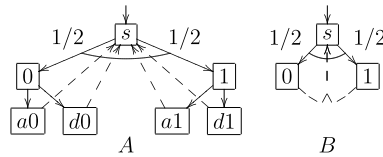
Fig. 7. Player A tries to guess if the outcomes agree.
