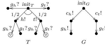
Fig. 11. T tosses a coin, G guesses heads or tails.
