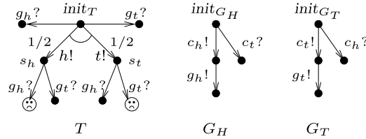
Fig. 12. Two different guessers.
