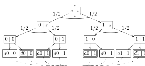
Fig. 8. MDP obtained by composing A and B.
