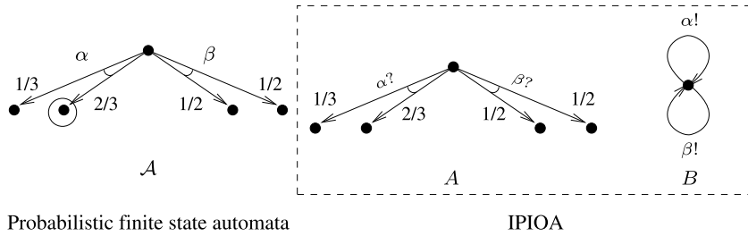
Fig. 6. From PFA to IPIOA.
