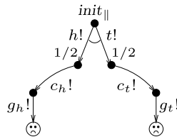
Fig. 13. A dubious scheduling.
