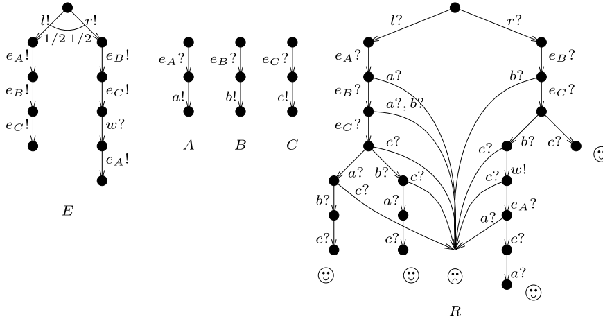
Fig. 4. Example showing that randomisation adds power to strongly distributed schedulers.
