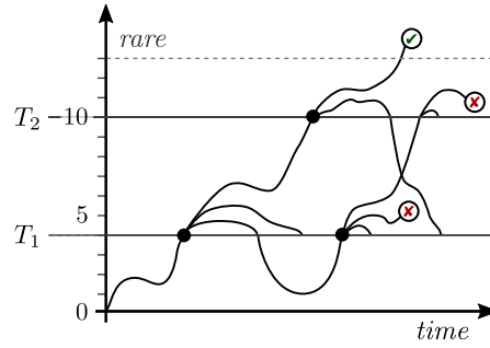
Fig. 2. RESTART.
