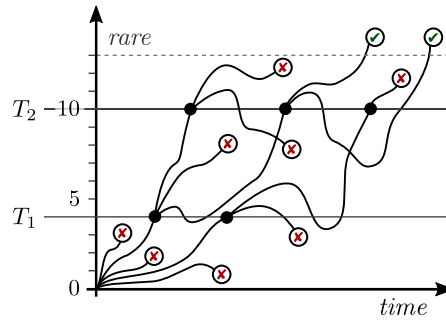
Fig. 3. Fixed effort.
