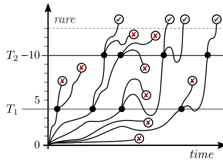
Fig. 4. Fixed success.
