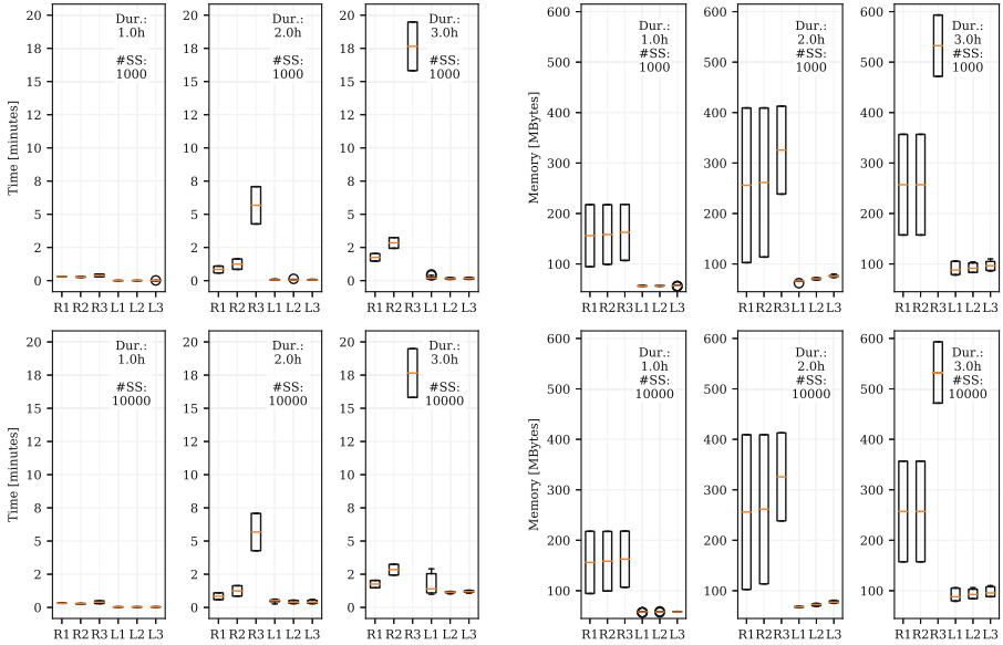
Fig. 8. Solving time (left) and memory (right) for RRRN for different source-target nodes, contact plan durations, and numbers of schedulers sampled (R: RUCoP, L: LSS).
