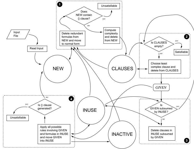
Figure 2: The “given clause” algorithm
