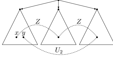
Figure 16: Example of (hypothetical) “gluing”.
