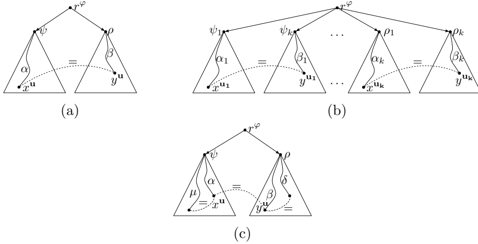
Figure 4: (a) A witness for \langle \downarrow[\psi]\alpha = \downarrow[\rho]\beta \rangle ; (b) we repeat the process of (a) for each conjunct \langle \downarrow[\psi_1]\alpha_1 = \downarrow[\rho_1]\beta_1 \rangle, \dots, \langle \downarrow[\psi_k]\alpha_k = \downarrow[\rho_k]\beta_k \rangle of \varphi ; (c) by adding a witness for \langle \downarrow[\psi]\alpha = \downarrow[\rho]\beta \rangle , we may be creating an unwanted witness for \langle \downarrow[\psi]\mu = \downarrow[\rho]\delta \rangle .
