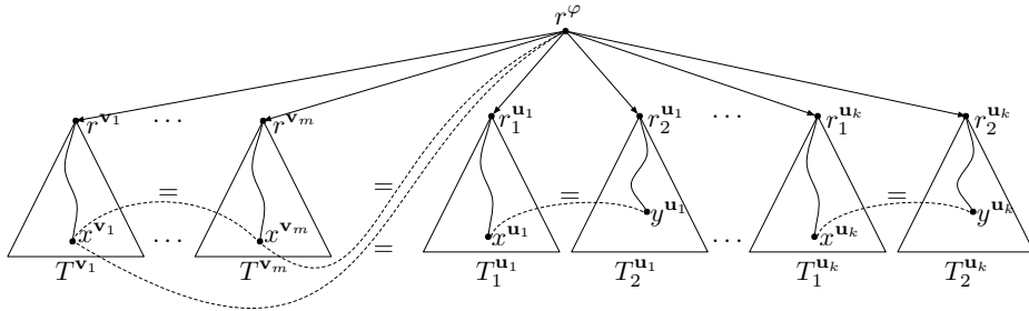
Figure 7: The data tree \mathcal{T}^\varphi , with root r^\varphi , when \mathbf{V} = \{\mathbf{v}_1, \dots, \mathbf{v}_m\} and \mathbf{U} = \{\mathbf{u}_1, \dots, \mathbf{u}_k\} . Nodes r^\varphi, x^{\mathbf{v}_1}, \dots, x^{\mathbf{v}_m} are in the same equivalence class, and for each i nodes x^{\mathbf{u}_i} and y^{\mathbf{u}_i} are in the same equivalence class.
