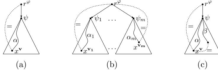
Figure 3: (a) A witness for \langle \epsilon = \downarrow[\psi]\alpha \rangle ; (b) we repeat the process of (a) for each conjunct \langle \epsilon = \downarrow[\psi_1]\alpha_1 \rangle, \dots, \langle \epsilon = \downarrow[\psi_m]\alpha_m \rangle of \varphi ; (c) by adding a witness for \langle \epsilon = \downarrow[\psi]\alpha \rangle , we may be creating an unwanted witness for \langle \epsilon = \downarrow[\psi]\beta \rangle .
