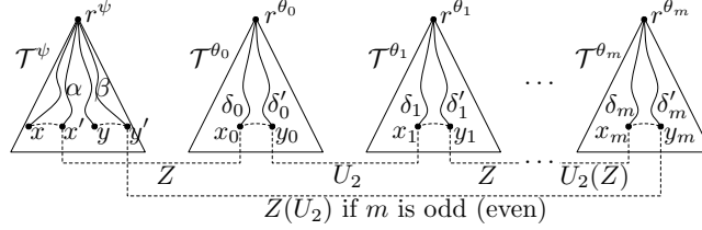
Figure 17: The hypothesis of Lemma 50
