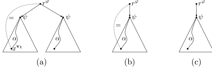
Figure 9: (a) Witnesses for \langle \epsilon = \downarrow[\psi]\alpha \rangle and \langle \epsilon \neq \downarrow[\psi]\alpha \rangle for (\psi, \alpha) \in \mathbf{V}_{=, \neq} ; (b) A witness for \langle \epsilon = \downarrow[\psi]\alpha \rangle for (\psi, \alpha) \in \mathbf{V}_{=, \neg \neq} ; (c) A witness for \langle \epsilon \neq \downarrow[\psi]\alpha \rangle for (\psi, \alpha) \in \mathbf{V}_{\neg =, \neq} .
