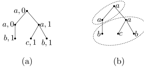
Figure 2: (a) A data tree. Nodes are tagged with (\ell, n) meaning that its label is \ell and its data-value is n . (b) Our view of data tree: a node-labeled tree and a partition over its nodes.
