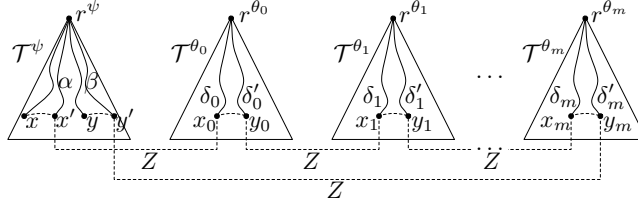
Figure 15: The hypothesis of Lemma 48
