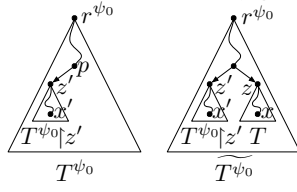
Figure 11: T = T^{\psi_0} \upharpoonright z is a new subtree with a special node x such that its class of data values is disjoint to the rest of \widetilde{\mathcal{T}}^{\psi_0} and \widetilde{\mathcal{T}}^{\psi_0}, \widetilde{r}^{\psi_0}, x \models \alpha .
