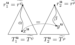
Figure 6: The data trees \mathcal{T}_1^{\mathbf{u}} = (T_1^{\mathbf{u}}, \pi_1^{\mathbf{u}}) and \mathcal{T}_2^{\mathbf{u}} = (T_2^{\mathbf{u}}, \pi_2^{\mathbf{u}}) for some \mathbf{u} \in \mathbf{U} . \pi^{\mathbf{u}_1} and \pi^{\mathbf{u}_2} are disjoint except that the equivalence class of x^{\mathbf{u}} is merged with the equivalence class of y^{\mathbf{u}} .
