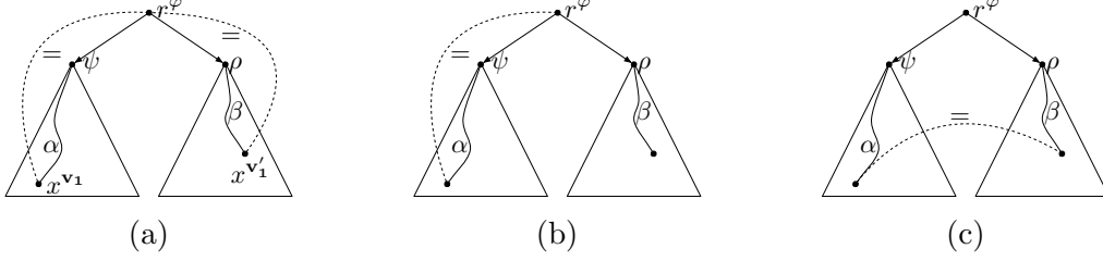
Figure 10: For (\psi, \alpha), (\rho, \beta) \in \mathbf{V}_{=, \neq} , (a) Witnesses for \langle \downarrow[\psi]\alpha = \downarrow[\rho]\beta \rangle ; (b) Witnesses for \langle \downarrow[\psi]\alpha \neq \downarrow[\rho]\beta \rangle ; For (\psi, \alpha) \in \mathbf{V}_{=, \neq}, (\rho, \beta) \in \mathbf{V}_{\neg=, \neq} or (\psi, \alpha), (\rho, \beta) \in \mathbf{V}_{\neg=, \neq} (c) Witnesses for \langle \downarrow[\psi]\alpha = \downarrow[\rho]\beta \rangle .
