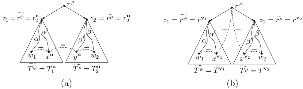
Figure 8: Nodes w_1 and w_2 are in the same equivalence class because (a) Rule 2 was applied via \mathbf{u} = (\psi, \alpha', \rho, \beta') \in \mathbf{U} , or (b) Rule 1 was applied twice via \mathbf{v}_1 = (\psi, \alpha'), \mathbf{v}_2 = (\rho, \beta') \in \mathbf{V} .
