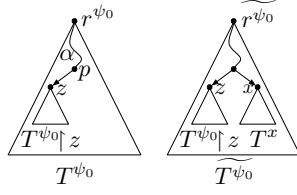
Figure 5: T^x = T^{\psi_0} \upharpoonright z is a new subtree with disjoint data values to the rest of \widetilde{T}^{\psi_0} . The new node x satisfies \widetilde{T}^{\psi_0}, r^{\psi_0}, x \models \alpha .
