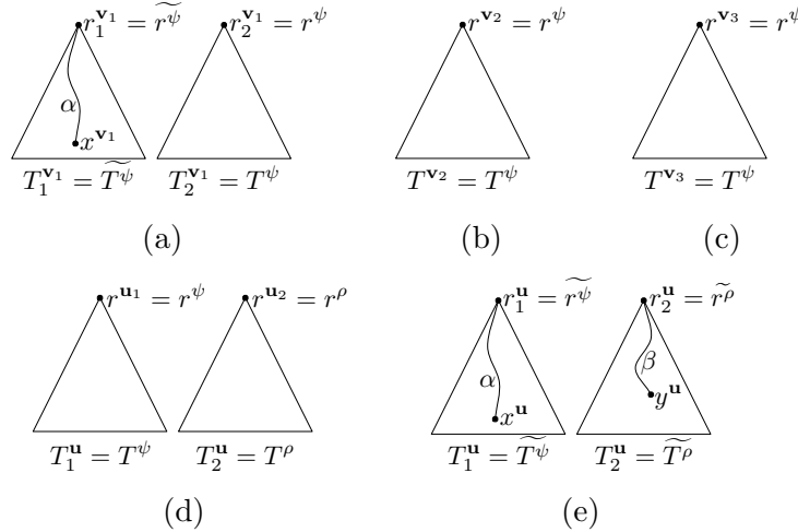
Figure 12: Witnesses for (a) \mathbf{v}_1 = (\psi, \alpha) \in \mathbf{V}_{=, \neq} ; (b) \mathbf{v}_2 = (\psi, \alpha) \in \mathbf{V}_{=, \neq} ; (c) \mathbf{v}_3 = (\psi, \alpha) \in \mathbf{V}_{\neq, =} ; (d) \mathbf{u} = (\psi, \alpha, \rho, \beta) \in \mathbf{U}_1 ; (e) \mathbf{u} = (\psi, \alpha, \rho, \beta) \in \mathbf{U}_2 .
