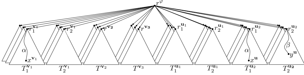
Figure 13: The tree T^\varphi (without any partition yet).
