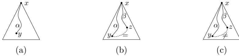
Figure 1: In x it holds: (a) The modal diamond \langle \alpha \rangle ; (b) the data-aware diamond \langle \alpha = \beta \rangle ; (c) the data-aware diamond \langle \alpha \neq \beta \rangle ;
