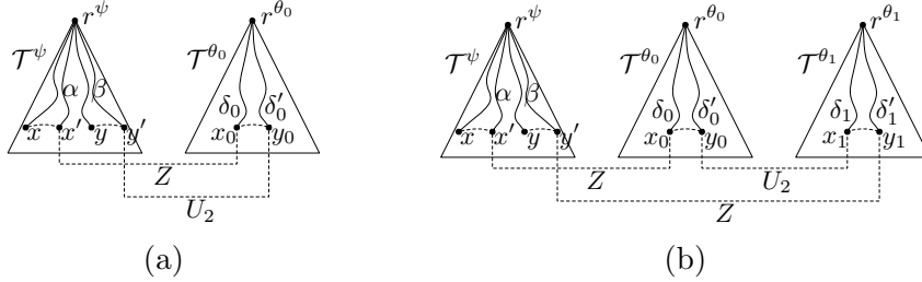
Figure 18: Proof of Lemma 50. (a) case m = 0 . (b) case m = 1 .
