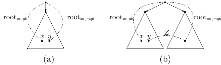
Figure 14: Examples of (hypothetical) “gluings”.
